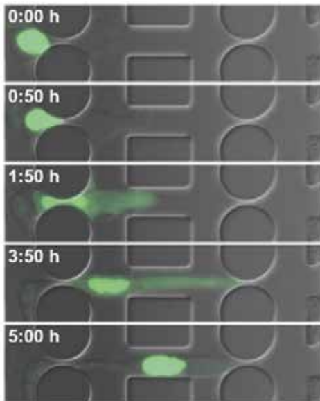
A live cell fluorescence microscopy image sequence showing a cancer cell undergoing nuclear envelope rupture during migration through a constriction, visualized by green fluorescent protein spilling from the nucleus into the cytoplasm.
